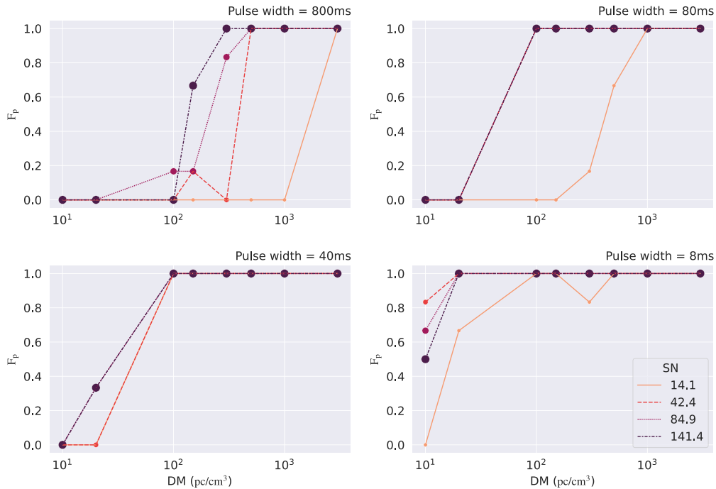
Figure 9. The fraction of recovery of single pulses ( F_p ) as a function of DM for multiple widths in an RFI environment which has a 2\sigma level of broad-band RFI affecting 10 per cent of total time samples observed. The result is similar to Fig. 6 which indicates that the ZDMF algorithm is unaffected by the amount of broad-band RFI in the data.
