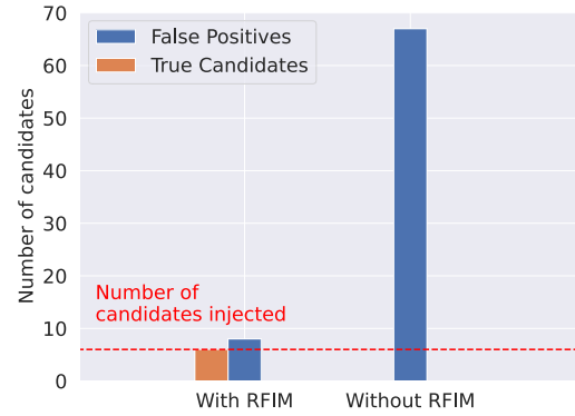
Figure 3. Histogram of the number of true and false positive candidates detected with and without RFIM in a single pulse search. A test vector containing six pulses with a DM of 300 \text{ pc cm}^{-3} , a width of 40 ms, a single-pulse S/N of 42.4, and a combination of all three types of RFI ( 2\sigma ) is searched for single pulses. Once without RFI cleaning and once after cleaning using IQRM and ZDMF.
