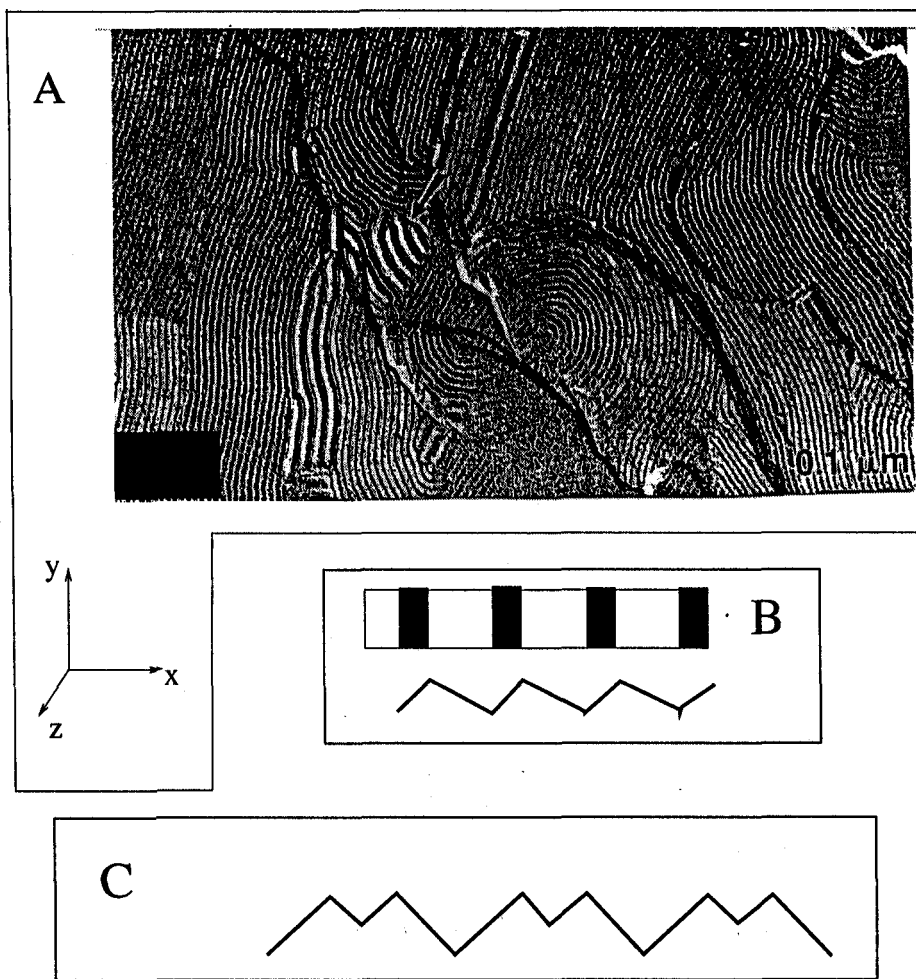
Figure 1.11: (A): A typical Freeze Fracture micrograph of the ripple phase (DPPC). A small patch of A ripples is indicated by an arrow. (from ref. [24]). The height modulation direction is in the plane of the paper. (B): The black and white bands in the figure correspond to the two arms of the saw-tooth-like (or triangular-like) ripples. (C): The non-centrosymmetric “M”-shape for the A ripples predicted by freeze fracture.
