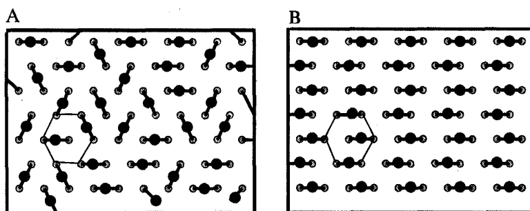
Figure 1.5: The small dots represent the chains that are arranged on a triangular lattice. The bigger dots represent the head-groups that are disordered in the L_{\beta'} phase (A) but get ordered in the L_{C'} phase (B).
