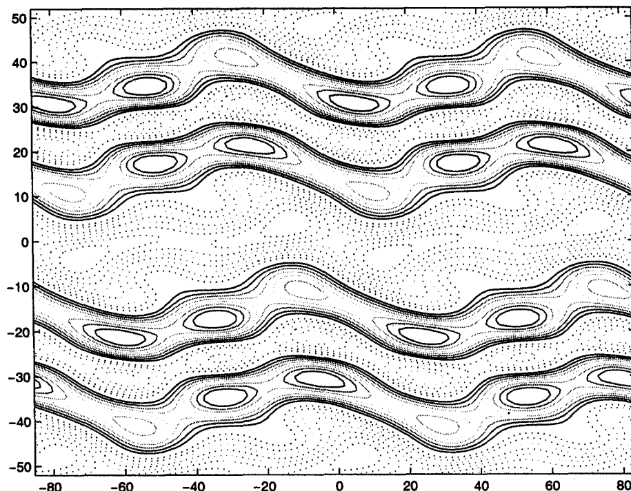
Figure 1.10: Electron density map of DLPC at -7°C and 77% by weight of water, calculated using the phases given in ref. [5].
