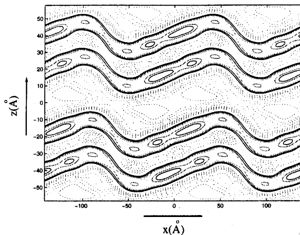
Figure 1: Electron Density Map of the ripple phase of DMPC. Temperature = 18.2^{\circ}\text{C} and partial specific volume of water = 0.263. The positive (negative) contours are represented by solid (dotted) lines. The regions with positive electron density correspond to the head-groups. Note that the thickness of the bilayers is about 40 Å, whereas that of the water region is about 15 Å.
