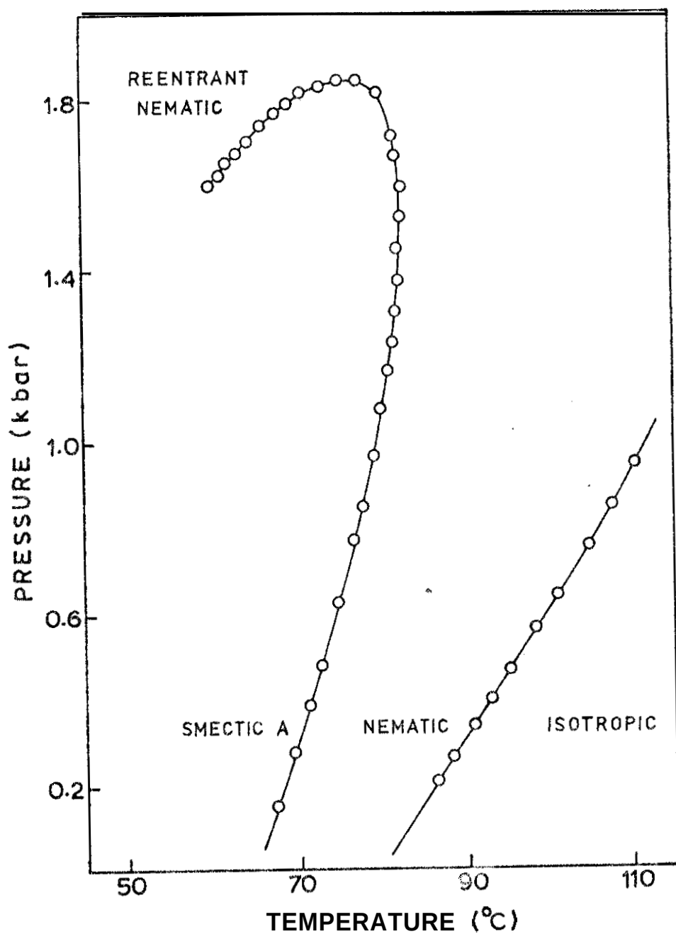
FIGURE 3.4: P-T Diagram of 8 OCB showing the isotropic nematic, smectic A and re-entrant nematic phases in the cooling mode. (After Cladis et al. 4 ).
