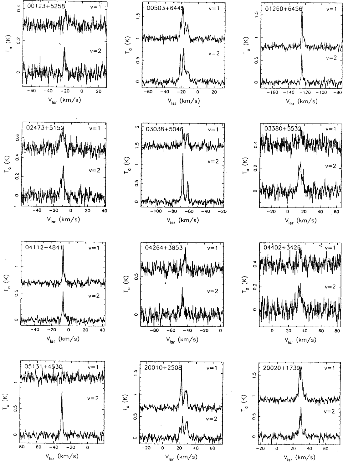
Fig. 1. Spectra of 21 ^{28}\text{SiO} new detections. The x-axis labels the velocity in LSR (Local Standard of Rest); the y-axis the intensity in antenna temperature, v at right side of the emission line, the vibrational state of the SiO maser line.
