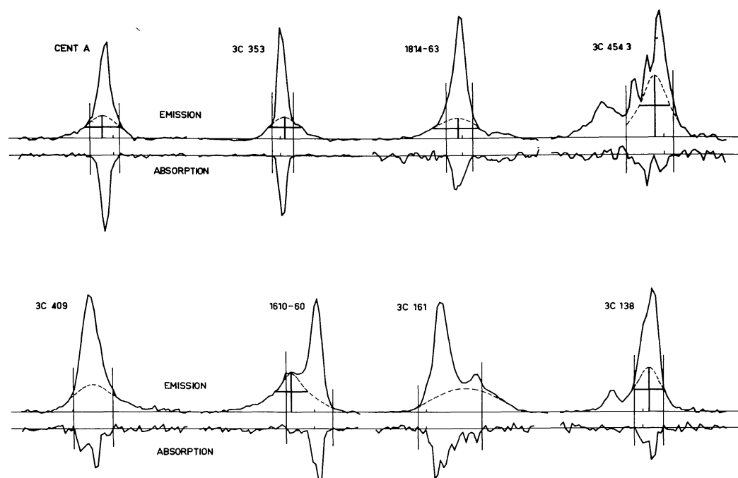
Fig. 2. Comparison of eight emission and absorption spectra obtained at intermediate latitudes and selected on the basis of high signal-to-noise ratio. The velocity limits of the absorption spectra are demarcated, showing clearly the presence of an optically thin component in every emission spectrum. These low, wide components are shown by dashed lines, and in some cases (crosses) their parameters can be determined by a computer analysis into Gaussians.
