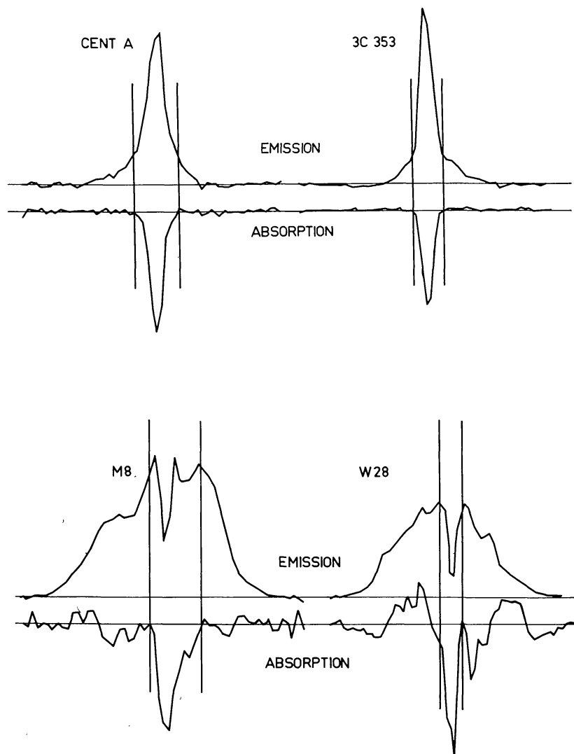
Fig. 6. (Upper) 21-cm emission and absorption spectra obtained in the directions of two intermediate-latitude sources ( b \approx 20^\circ ). The absorption in both cases corresponds to the peaks in the emission profiles caused by low-temperature, high-opacity concentrations of hydrogen. The wings of the emission profiles are from the optically thin high-temperature medium and are not seen in absorption.
