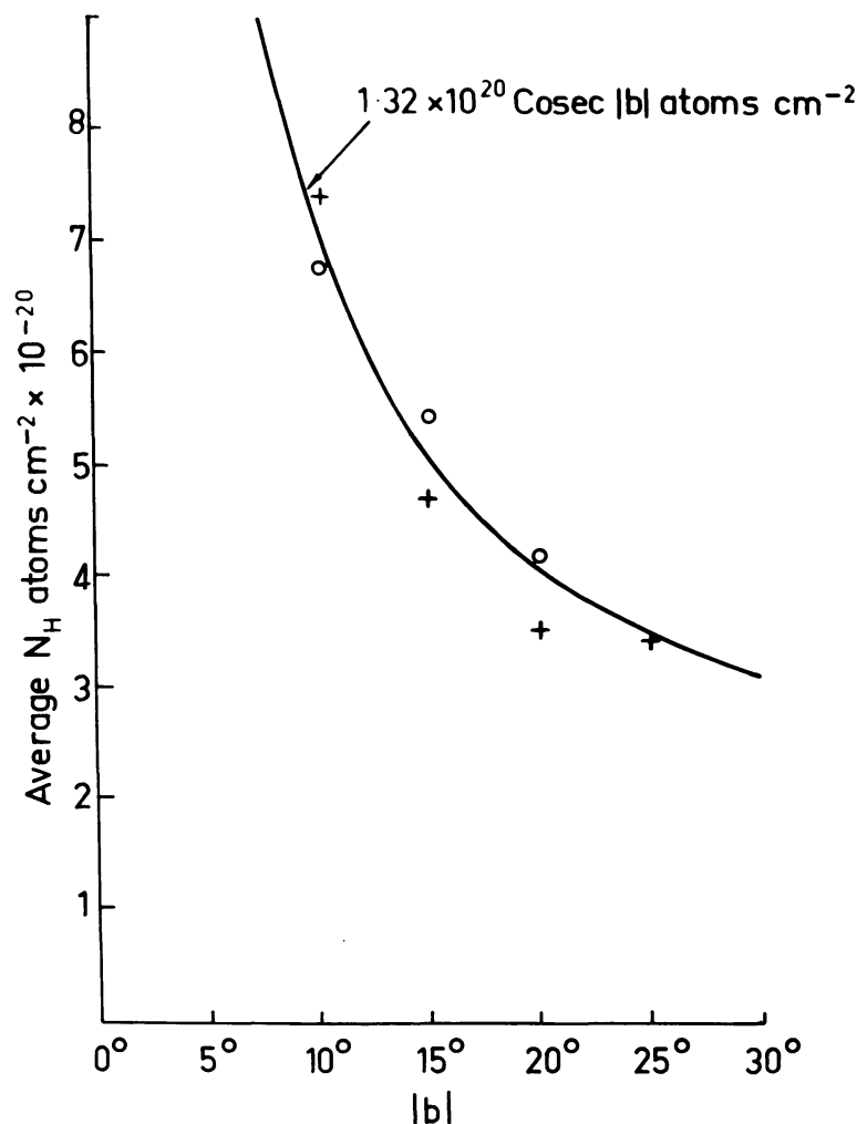
Fig. 1. The mean column density of the widest Gaussian component at each latitude observed by Takakubo and van Woerden (1966) is shown plotted as a function of the absolute value of the latitude. The crosses and circles refer to observations at north and south latitudes. The cosecant dependence on the latitude illustrates the stratified nature of the hydrogen distribution giving rise to the wide components in the profiles.
