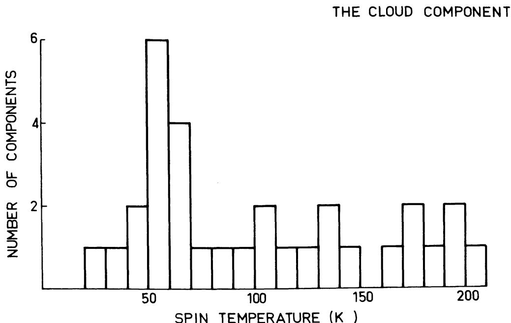
Fig. 5. A histogram of the calculated spin temperatures for the narrow Gaussian components observed in both emission and absorption. The mean for the distribution is around 80 K.
