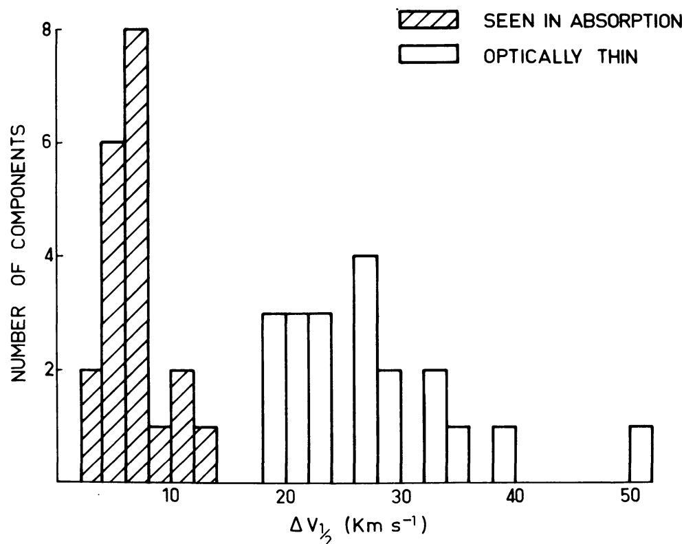
Fig. 3. A histogram of the number of Gaussian components as a function of their full widths observed in the direction of extragalactic sources at intermediate and high latitudes. A clear separation is evident between the narrow components with measurable optical depths and the wide optically thin components. The former originate in low-temperature concentrations and the latter in a high-temperature, widely dispersed medium.
