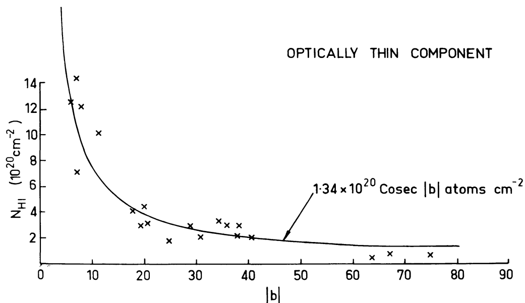
Fig. 4. The integrated column density in the wide optically thin component is shown plotted against the absolute value of the galactic latitude. The stratified nature of the hydrogen distribution giving rise to this component of the emission is shown by the fit to the cosecant curve.
