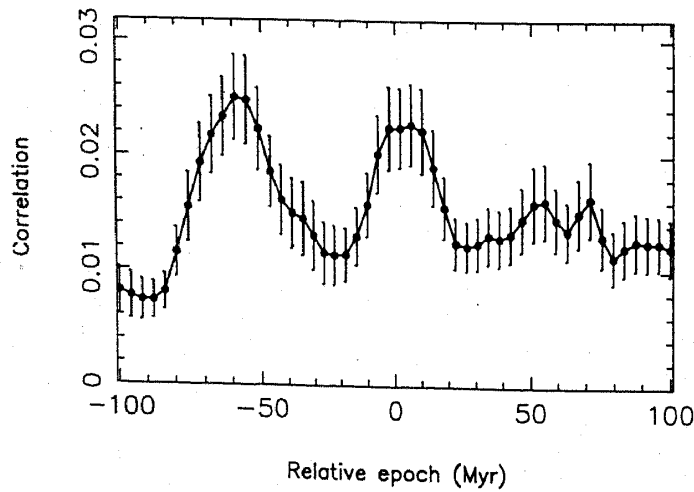
Figure 4. Plot of the correlation of the mass distribution in the spiral pattern at various epochs with the present pulsar distribution. This plot corresponds to a corotation resonance radius of 14 kpc. The error bars indicate 1\sigma deviation on either side. The locations of the peaks of the correlation correspond to an epoch which is 60 Myr ago and the present epoch.
