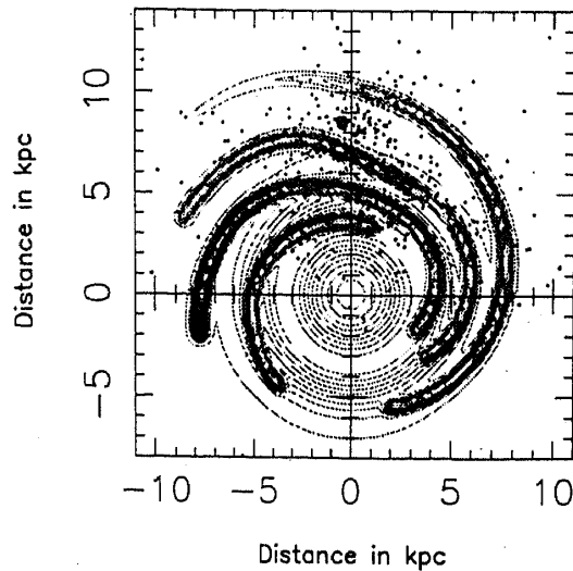
Figure 1. The new electron density distribution model of Taylor & Cordes (1993). Projected locations of all known pulsars are plotted as dots. Sun is at (0, 8.5).
