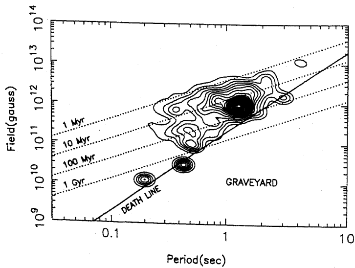
Figure 3. A contour representation of the distribution of 'true' number of pulsars as a function of pulsar period and magnetic field. The constant characteristic age lines corresponding to 1 Myr, 10 Myr, 100 Myr and 1 Gyr are also plotted. (From Deshpande et al. 1994. Reproduced by permission).
