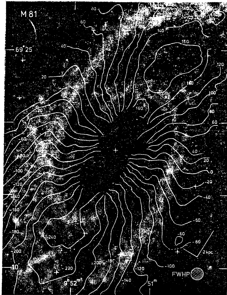
Figure 4. Measuring the dynamics of galaxies with the WSRT. This figure is from a thesis by H.C.D. Visser and shows the spiral galaxy M81. The contour lines in white represent the radial component of the motion of neutral hydrogen, as inferred from the Doppler effect. On a simple model of circular motion in a flat disc with a speed independent of radius, these contours would be straight lines through the centre. Striking deviations from this simple pattern near the spiral arms are seen, and these can be fitted by the 'density wave' theory.
