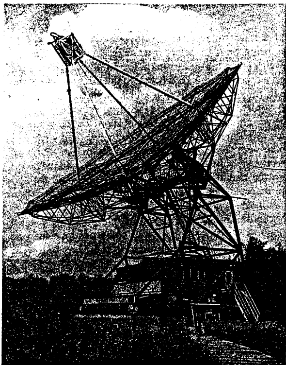
Figure 2. The 25 metre reflector at Dwingeloo in the Netherlands, completed in 1955, at which time it was the largest in the world. This telescope, light in weight (only 127 tonnes) and therefore of modest cost, was deliberately designed to study the interstellar (21 cm) hydrogen line.
