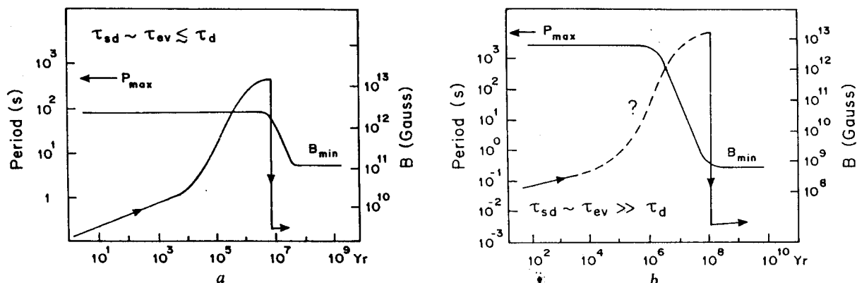
Figure 2. The rotational history and the evolution of the magnetic field of neutron stars in binaries. The first-born neutron star in a binary will be slowed down to very long periods owing to the electromagnetic torque exerted by the stellar wind from the companion. After the companion fills its Roche lobe, heavy accretion onto the neutron star will set in and in the process the neutron star will be spun up to an equilibrium period determined by its magnetic field and the accretion rate. After accretion stops, the spun-up neutron star will, once again, function as a pulsar. Figure a is appropriate for a massive companion whose evolution time ( \tau_{ev} ) is \lesssim \tau_d the ohmic dissipation timescale in the crust. In this case the decay of the field will lag behind the rapid period lengthening. The asymptotic field will be determined by the maximum period to which the neutron star was slowed down. Figure b is for the case when \tau_{ev} \gg \tau_d ; this may obtain in low-mass binaries. Here, field decay will 'track' the period of rotation.
