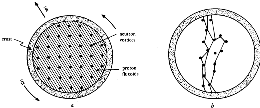
Figure 1. a, A view of the equatorial plane of a rotating neutron star showing an idealized geometry of the arrangement of the Onsager-Feynman vortices (parallel to the rotation axis) in the neutron superfluid and the Abrikosov vortices (parallel to the magnetic axis) in the proton superconductor. For the purpose of illustration the magnetic axis has been assumed to be perpendicular to the rotation axis. For the magnetic field to decay the fluxoids must migrate to the crust where, because of the finite conductivity, the field can decay. b, A more realistic state of affairs in the presence of strong interaction between the vortices in the two superfluids.
