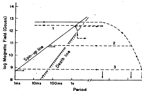
Figure 3. The evolution of neutron stars in the magnetic field-period plane. The curve labelled '1' corresponds to the case discussed in Figure 2 a ( \tau_{sd} \sim \tau_{ev} \lesssim \tau_d ). Curves '2' and '3' refer to two different situations in both of which \tau_{sd} > \tau_d . The 'spin-up line' is the equilibrium period line corresponding to accretion at the maximum possible Eddington rate. The 'death line' represents the turn-off of pulsar activity.
