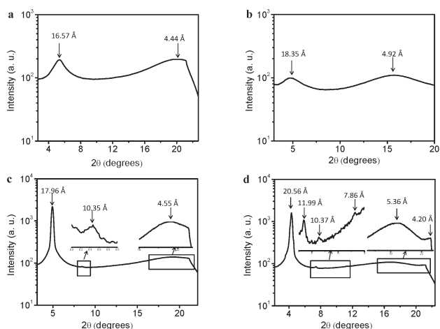
Fig. 2 The intensity profile of the X-ray pattern exhibited by PE-CB (a), PE-Ch (b), PE-TP (c), and PE-R (d) at 80 °C, 130 °C, 90 °C and 140 °C, respectively. See ESI† (Fig. S17) for X-ray diffractions pattern obtained at those temperatures.
