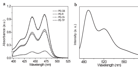
Fig. 3 (a) UV/vis absorption spectra of PE-CB , PE-R , PE-Ch and PE-TP in \text{CHCl}_3 . (b) Representative fluorescence spectra of PE-CB in \text{CHCl}_3 .
