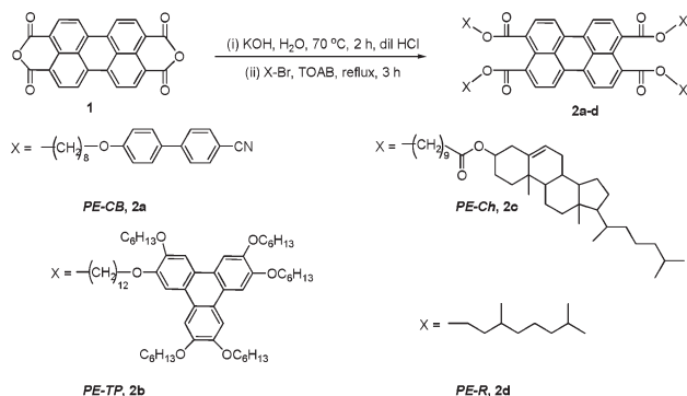
Scheme 1 Synthesis of perylene-based non-conventional LCs.
