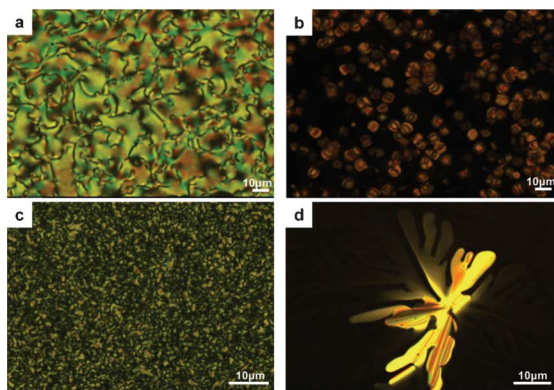
Fig. 1 Optical photomicrograph of compounds (a) 2a (b) 2b (c) 2c and (d) 2d at 80 °C, 100 °C, 125 °C and 140 °C, respectively (on cooling, crossed polarizers, scale bar 10 μm).
