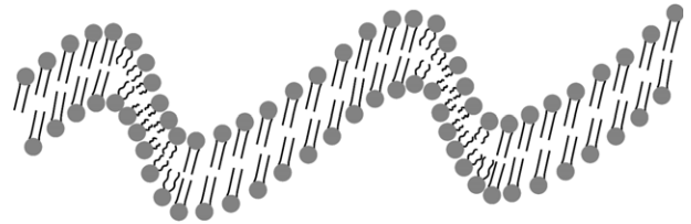
Fig. 5: Schematic of the bilayer profile obtained from the model. Note that the bilayer thickness is different in the two arms of the saw-tooth-like ripples.
