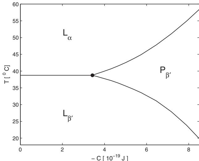
Fig. 3: Phase diagram in the C - T plane calculated from the model. a'_2 = 159.42 k_B , T^* = 260 K. Values of the other coefficients in units of k_B T^* are: a_3 = -306.5 , a_4 = 613.15 , b_2 = 0.2 , b_4 = 200 , D = 557.41 , E = 600 , \Gamma_1 = 0.010 , \Gamma_2 = 1.80 , \Gamma_3 = 500 , \Gamma_4 = -3 , \Gamma_5 = -20 , \Gamma_6 = -20 , \Gamma_7 = -50 , \Gamma_8 = -25 . Both the main transition ( L_\alpha \rightarrow L_{\beta'} ; L_\alpha \rightarrow P_{\beta'} ) and pre-transition ( P_{\beta'} \rightarrow L_{\beta'} ) are first order.
