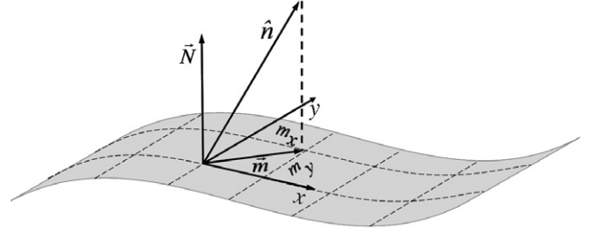
Fig. 2: The unit vector \mathbf{n} represents the orientation of the long axis of the lipid molecules relative to \mathbf{N} , the bilayer normal. \mathbf{m} = \mathbf{n} - (\mathbf{N} \cdot \mathbf{n}) \mathbf{N} is the projection of \mathbf{n} on the bilayer plane.
