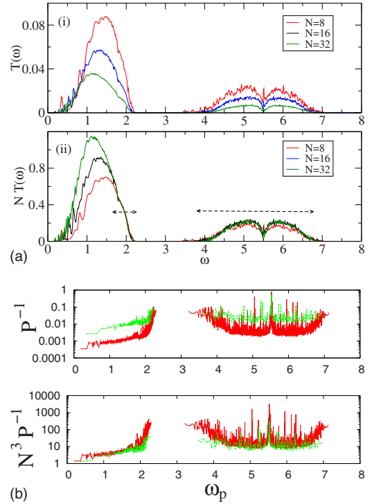
FIG. 16. (Color online) 3D unpinned case with fixed BC for \Delta=0.8 . Top: plot of the disorder-averaged transmission T(\omega) versus \omega . The inset shows the same data multiplied by a factor of N . Bottom: plot of the IPR ( P^{-1} ) and scaled IPR ( N^3 P^{-1} ) as a function of normal-mode frequency \omega_p for a fixed disorder realization. The curves are for N=8 (green) and 16 (red).
