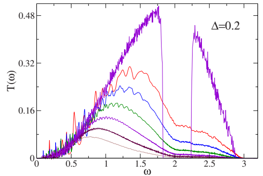
FIG. 7. (Color online) 2D unpinned case with fixed BC for \Delta = 0.2 . Plot of the disorder-averaged transmission T(\omega) versus \omega . The uppermost curve corresponds to a binary-mass ordered lattice with N=128 while the remaining curves (from top to bottom) correspond to square lattices with N=16, 32, 64, 128, 256 , and 512 , respectively.
