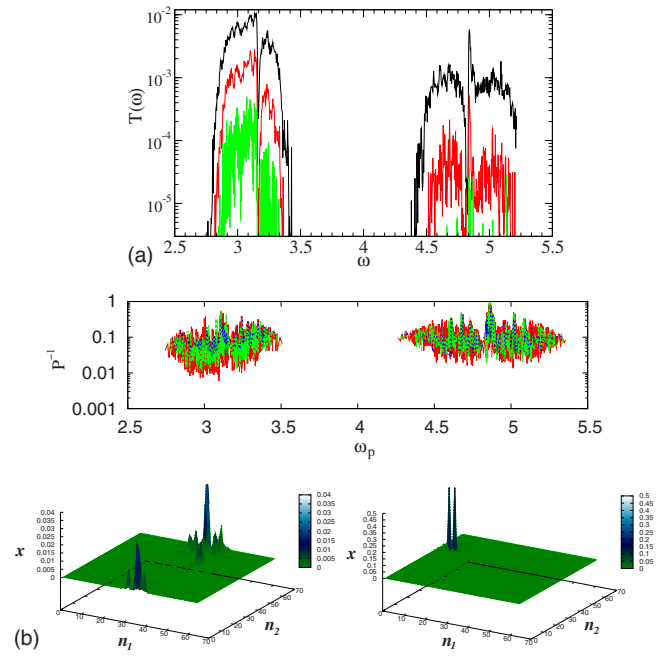
FIG. 13. (Color online) 2D pinned case for \Delta=0.4 and k_o=10.0 . Top: plot of the disorder-averaged transmission T(\omega) versus \omega . The various curves (from top to bottom) correspond to lattices with N=16, 32 , and 64 , respectively. Here we choose \gamma=\sqrt{10} . Bottom: plot of the IPR ( P^{-1} ) as a function of normal-mode frequency \omega_p . The curves are for N=16 (blue), 32 (green), and 64 (red). Also shown are two typical normal modes for one small (left) and one large value of P^{-1} for N=64 .
