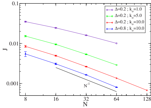
FIG. 25. (Color online) 3D pinned case. Plot of disorder-averaged current J versus system size for different values of k_o and \Delta . The data sets for \Delta=0.2 for different values of k_o are from simulations while the data for \Delta=0.8 is from numerics.
