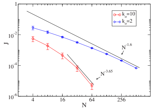
FIG. 14. (Color online) 2D pinned case for \Delta=0.4 . Plot of disorder-averaged current J versus system size for two different values of k_o . Error bars show standard deviations due to disorder and numerical errors are much smaller. Note that the standard deviation do not decrease with system size for higher k_o .
