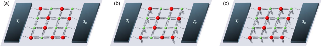
FIG. 1. (Color online) A schematic diagram of a two-dimensional mass-disordered lattice of particles connected by harmonic springs and connected to heat baths at temperatures T_L and T_R . Red and green colors indicate particles of different masses. Pinning refers to the presence of a spring attaching a particle to the substrate. In (a) there is no pinning, in (b) boundary particles are pinned, and in (c) all sites are pinned.
