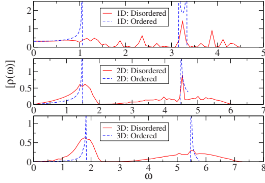
FIG. 3. (Color online) Unpinned lattices with fixed BC in one direction and periodic in all others. Disorder-averaged density of states obtained numerically from the eigenvalues of several disorder realizations in 1D, 2D, and 3D for lattice sizes N=4096 , 64, and 16, respectively. Note that the low-frequency behavior is unaffected by disorder and one has \omega^{d-1} as \omega \rightarrow 0 . We set \Delta=0.8 , k=1 and averaged over 30 realizations in 1D and over 10 realizations in 2D and 3D. In 2D and 3D there is not much variation in \rho(\omega) for different disorder samples. Also shown are the density of states for the binary-mass ordered lattices.
