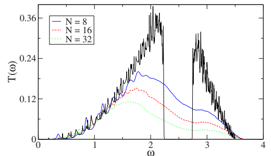
FIG. 17. (Color online) 3D unpinned case with fixed BC for \Delta=0.2 . Plot of the disorder-averaged transmission T(\omega) versus \omega . The uppermost curve is the transmission curve for the binary-mass ordered lattice for N=16 .
