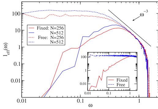
FIG. 12. (Color online) Plot of the effective mean-free path l_{\text{eff}}=NT(\omega)/\omega^{d-1} in 2D with \Delta=0.8 . The insets show l_{\text{eff}} for the ordered lattices with a single mass. An \omega^{-3} behavior is observed in a small part of the diffusive region. The fixed BC data is highly oscillatory and has been smoothed.
