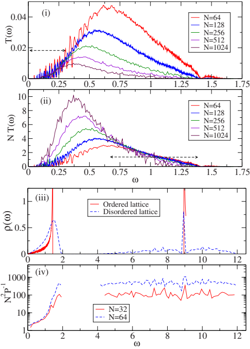
FIG. 5. (Color online) 2D unpinned case with fixed BC for \Delta = 0.95 . (i) Plot of the disorder-averaged transmission T(\omega) versus \omega . (ii) Plot of NT(\omega) . The range of frequencies for which T(\omega) \sim 1/N is indicated by the dashed line. (iii) Plot of \rho(\omega) for binary-mass ordered and single disordered sample. (iv) Plot of N^2P^{-1} for single samples (smoothed data). We see that even though allowed normal modes occur over a large frequency band \approx(0-12) , transmission takes place in a small band \approx(0-1.25) and is negligible elsewhere. The IPR plots confirm that the nontransmitting states correspond to localized modes. In (i) we see that \omega_c^L is slowly decreasing with increase in N .
