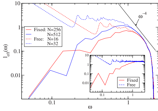
FIG. 22. (Color online) Plot of the effective mean-free path \ell_{\text{eff}}=NT(\omega)/\omega^{d-1} in 3D with \Delta=0.8 for fixed and free BCs. The insets show \ell_{\text{eff}} for the ordered system with a single mass. An \omega^{-4} behavior is observed in a small part of the diffusive region. The fixed BC data are highly oscillatory and has been smoothed.
