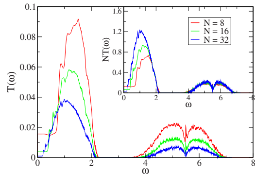
FIG. 21. (Color online) 3D unpinned case with free BC for \Delta=0.8 . Top: plot of the disorder-averaged transmission T(\omega) versus \omega . The inset shows the same data multiplied by a factor of N .
