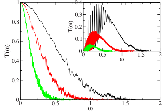
FIG. 2. (Color online) 1D unpinned case with both free and fixed (inset) boundary conditions: plot of the disorder-averaged transmission T(\omega) versus \omega for \Delta=0.4 . The various curves (from top to bottom) correspond to lattices of sizes N=64 , 256, and 1024, respectively.
