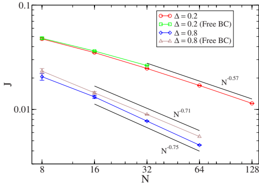
FIG. 18. (Color online) 3D unpinned case with fixed and free BCs. Plot of disorder-averaged current J versus system size for two different values of \Delta . The data for \Delta=0.2 are from simulations. The error bars show standard deviations due to disorder and numerical errors are smaller.
