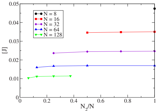
FIG. 19. (Color online) 3D unpinned case with fixed BC for \Delta=0.2 . Plot of disorder-averaged current density J (with the definition J=I/N_2^2 ) versus N_2/N for different fixed values of N . We see that the 3D limiting value is reached at quite small values of N_2/N .
