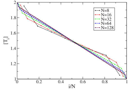
FIG. 20. (Color online) 3D unpinned case with fixed BC for \Delta=0.2 . Plot of temperature profile T_i in a single disorder realization for different system sizes. The plots are from simulations.
