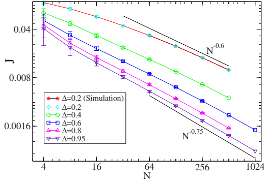
FIG. 8. (Color online) 2D unpinned lattice with fixed BC. Plot of disorder-averaged current J versus system size for different values of \Delta . The error bars show the actual standard deviations from sample-to-sample fluctuations. Numerical errors are much smaller. For \Delta=0.2 , simulation data are also plotted.
