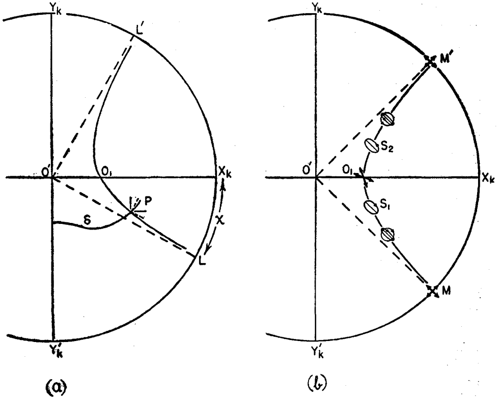
TEXT-FIG. 3. (a) Curvilinear co-ordinates ( \delta, \chi ) for the point P in the convergent light figure. (b) States of polarisation of the waves propagated along directions represented by points on MO_1M' ; S_1 and S_2 are the singular axes.
