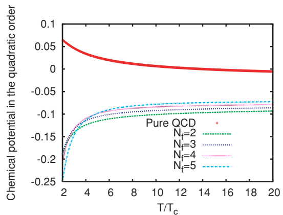
FIG. 6. (Color online) Effective chemical potentials at the quadratic order for EOS2.
