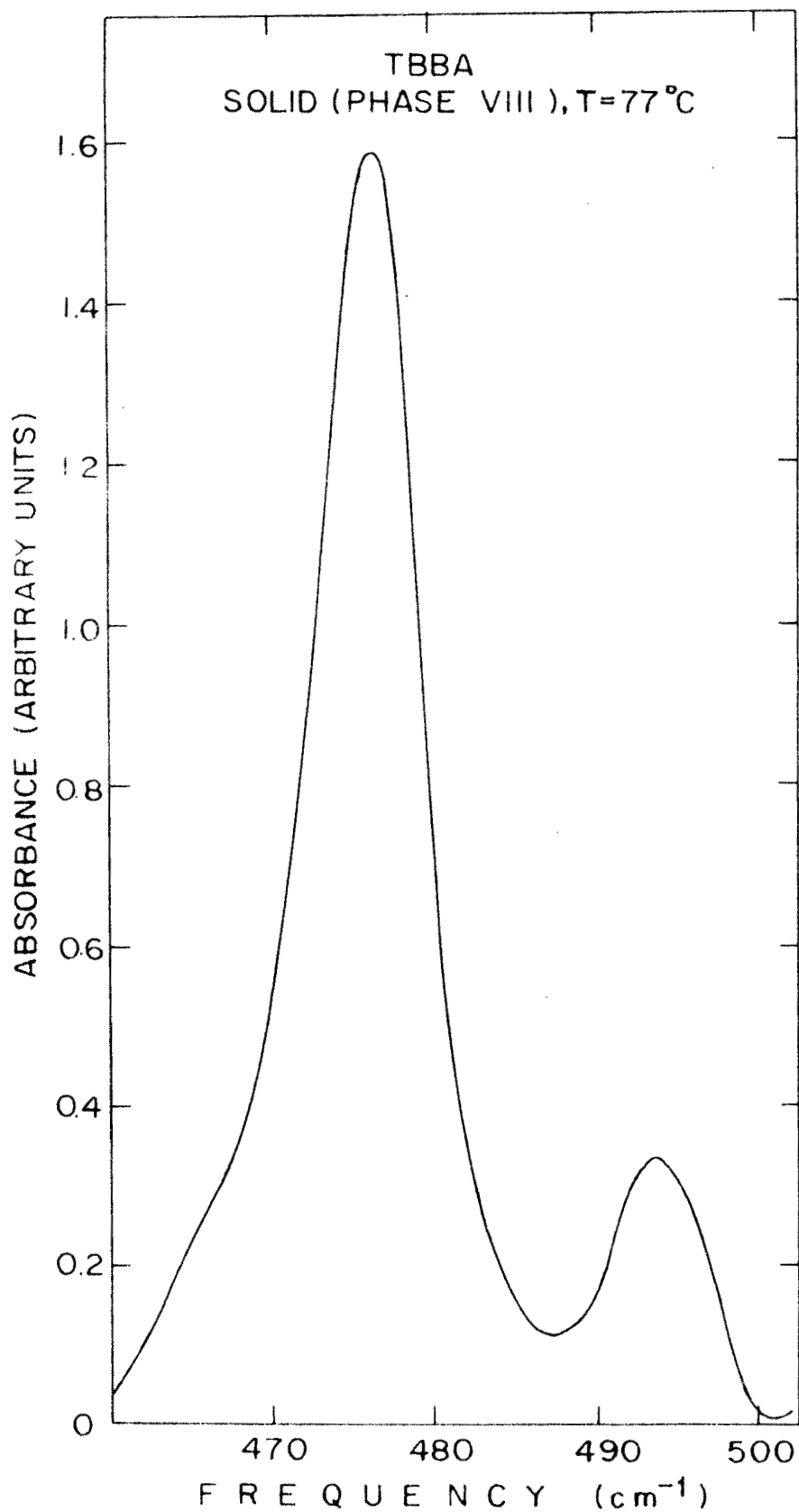
FIGURE 5.4: Absorbance of the solid phase of TBBA (T = 77°C) in the spectral interval 460-500 cm -1 .
