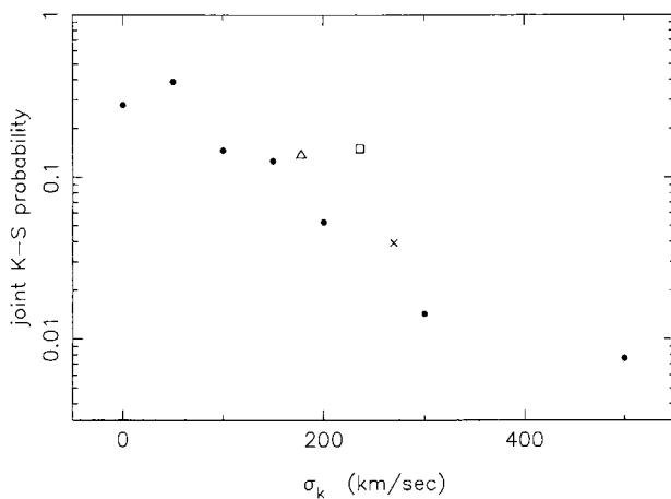
Figure 2. The distribution of maximum joint KS probabilities for LMXBs as a function of \sigma_k . The dots indicate Maxwellian kick speed distributions of \sigma_k = 0, 50, 100, 150, 200, 300 and 500 \text{ km s}^{-1} (the root mean square speed of a Maxwellian distribution is \sqrt{3} \times \sigma_k ). The LL, Paczyński and HPP distributions are indicated by the cross, triangle and square, with average speeds of 430, 284 and 376 \text{ km s}^{-1} , respectively. For these three distributions, the x-axis value indicates \sqrt{\pi/8} times the average speed.
