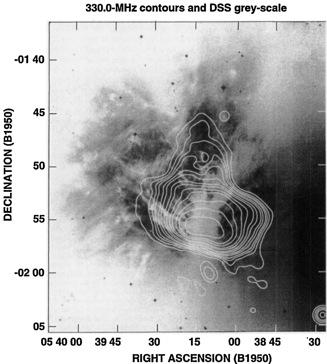
Figure 1. Contour representation of the 330-MHz image of NGC 2024 made with a beam of FWHM 65.1 \times 64.6 arcsec 2 at a position angle (PA) of 61^\circ.2 . Contours are at 10 mJy beam -1 \times (-2, 2, 4, 6, 8, 12, 16, 24, 32, 48, 64, 96, 128, 192) . An optical image of NGC 2024 is shown in grey-scales.
