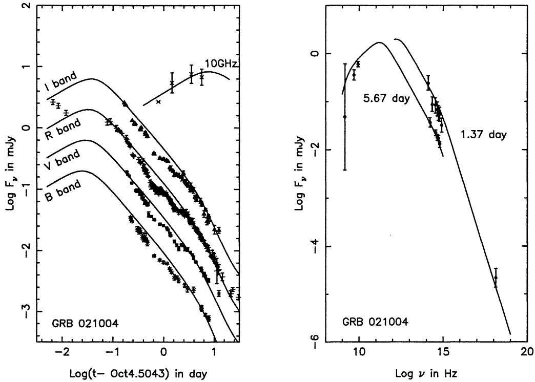
Figure 3. Multi-band observed light curves (left panel) and broadband spectrum (right panel) of the GRB 021004 OA are compared with model predictions shown as solid curves. A total extinction of E(B-V)=0.20 mag has been used. For clarity of display, in the left panel the B, V, I and radio light curves are shifted vertically by -1.0, -0.5, +0.5 and +1.0 respectively in logarithmic scale. The radio light curve at 10 GHz is constructed, by extrapolation with expected spectral slope, from measurements reported at 22.5 GHz, 15 GHz and 8.46 GHz at different epochs (Frail & Berger 2002, Pooley et al. 2002, Berger et al. 2002). The frequency of 10 GHz was chosen to correspond with a similar plot presented by Kobayashi & Zhang (2003). The model uses \nu_a = 2.1 GHz, \nu_m = 2.5 \times 10^{14} Hz and \nu_c = 3.3 \times 10^{16} Hz at t = 0.06 day; a jet break time t_b = 6.7 day and an electron energy distribution index p = 2.27 . The model includes the host galaxy contribution estimated in section 3.2. In the right panel an expected spectrum with p = 2.27 is shown with the Chandra HETG measurement (Sako & Harrison 2002a) and optical and near-IR observations at the same epoch, \sim 1.37 day. A similar spectrum is also shown at t = 5.67 day, the epoch of the cm-wave radio observations reported by Berger et al. (2002). Where necessary, fluxes measured at optical, near-IR and radio wavelengths were interpolated between adjacent data points at one wavelength in order to determine a contemporaneous value with another wavelength.
