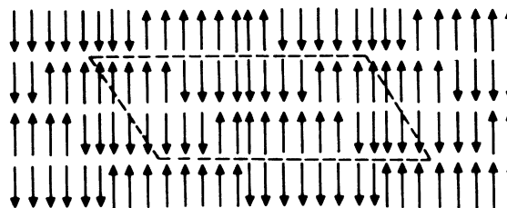
FIG. 10. A highly simplified schematic model of the smectic- \tilde{C} structure. A very small tilt of the director with respect to the layer normal has been ignored; this angle is much smaller than that typically seen in \text{Sm-}C_2 phases. The arrows indicate the polar end groups. Note that the local polar ordering is predominantly \text{Sm-}A_2 -like, but the polarization modulation is tilted with respect to the molecular layers. The oblique centered \text{Sm-}\tilde{C} lattice can be considered as a “sheared” variant of the \text{Sm-}\tilde{A} structure.
