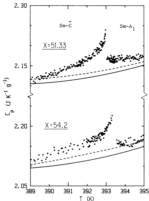
FIG. 6. Detailed view of the C_p variation near the \text{Sm-}A_1\text{-Sm-}\tilde{C} transition in samples with X = 51.33 and 54.2 . The solid and dashed curves represent the background curves shown in Figs. 2 and 3. Both these transitions are weakly first order, and data points in the narrow coexistence region are not shown.
