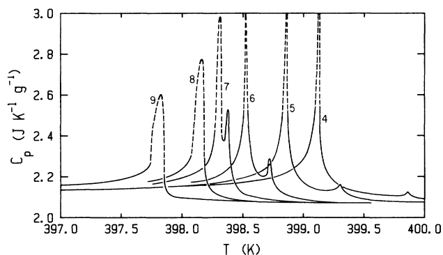
FIG. 9. The evolution of the heat capacity of the 51.33 mol % mixture in the \text{Sm-}A_d\text{-}N_r\text{-Sm-}A_1 region as a function of elapsed time. Run numbers are given; these runs were made following completion of three runs carried out under normal operating conditions (see text). The accumulated time above 400 K at the beginning of each run is (4) 86 h, (5) 126 h, (6) 167 h, (7) 193 h, (8) 206 h, and (9) 219 h. The dashed portions of curves indicate apparent C_p values obtained in a two-phase coexistence region.
