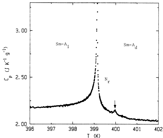
FIG. 7. The C_p variation in the \text{Sm-}A_d\text{-}N_r\text{-Sm-}A_1 transition region for the 51.33 mol % mixture. Note the very small \text{Sm-}A_d\text{-}N_r peak marked by the arrow. These data were obtained on a slow heating run (scan rate = +95 mK/h).
