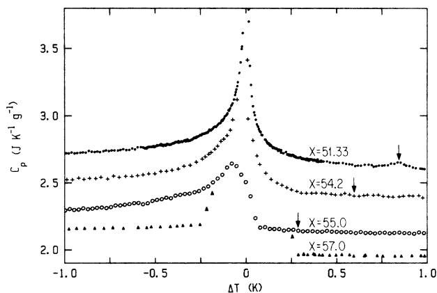
FIG. 8. Detailed view of the C_p variation associated with the N_r\text{-Sm-}A_1 transition ( X = 51.33, 54.2, \text{ and } 55.0 ) and the direct first-order \text{Sm-}A_d\text{-Sm-}A_1 transition ( X = 57.0 ). The data for X = 55.0, 54.2, \text{ and } 51.33 have been shifted by +0.1, +0.3, \text{ and } +0.5 \text{J K}^{-1} \text{g}^{-1} , respectively. The arrows mark the \text{Sm-}A_d\text{-}N_r transition observed for the 51.33 mol % sample and the position expected for the 54.2 and 55.0 mol % samples on the basis of microscope observations. In order to avoid confusion, only three data points in the two-phase coexistence region are shown for the 57.0 mol % sample. The transition temperatures used to determine \Delta T were T_c = 339.14 K (51.33 mol %), T_1 = 398.80 K (54.2 mol %), 398.20 K (55.0 mol %), and 397.85 K (57.0 mol %).
