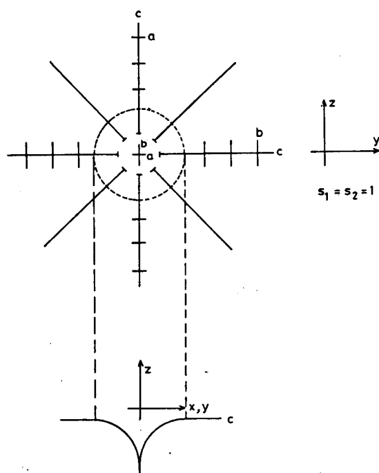
Figure 4. Removal of singularity in a hybrid with s_1 = s_2 = 1 by an escape in the c director through \pi/2 .
