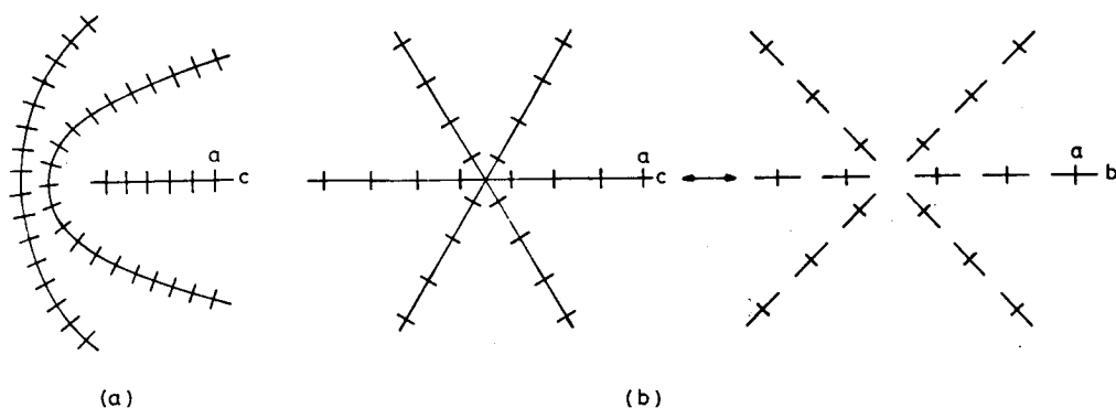
Figure 1a, b. (a) s = +\frac{1}{2} wedge disclination in a - c fields; (b) s = +1 wedge disclination in a - c fields can be transformed into an s = +1 wedge disclination in a - b fields by allowing the c director to escape in the third dimension.
