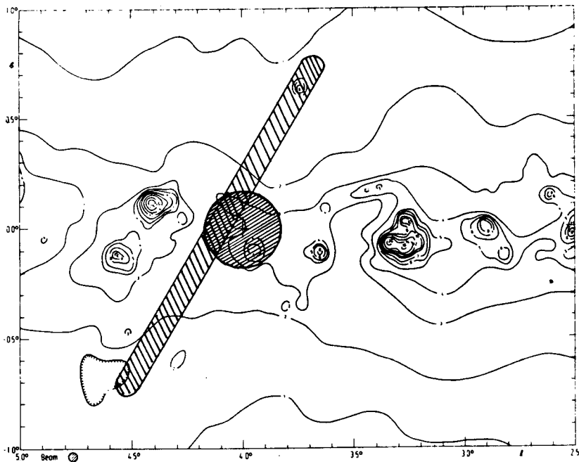
Figure 2. A typical blank region (see text) in the galactic plane for the beam used in the H 272 \alpha survey (elongated hatched area). The circular hatched area represents the beam used by Lockman (1976) who observed H 166 \alpha line at this position. The 5 GHz continuum map is from Altenhoff et al. (1978).
