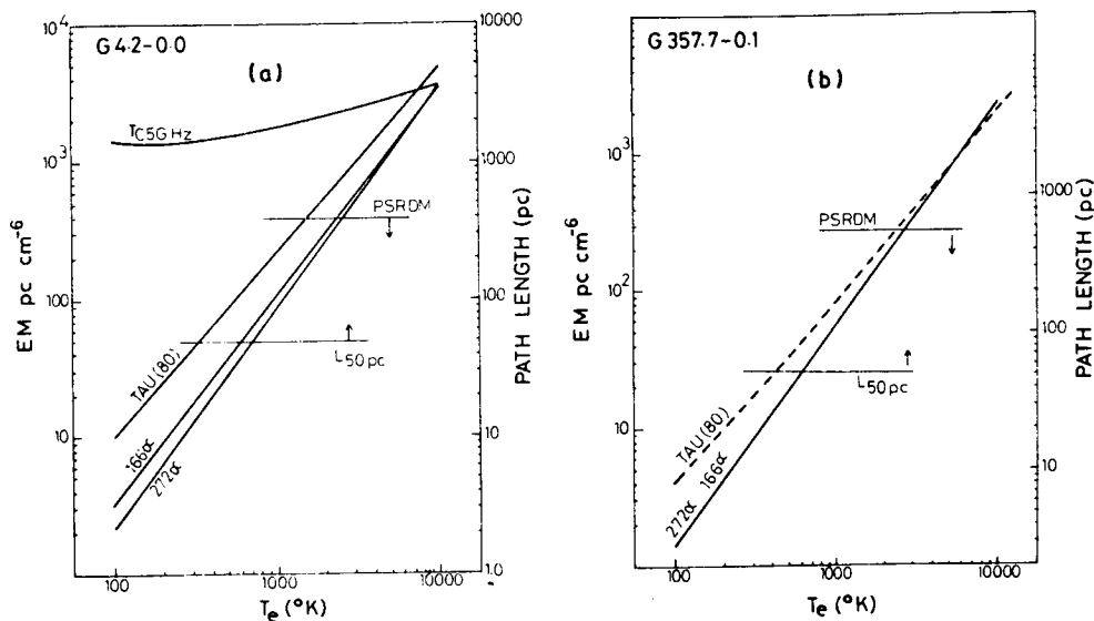
Figure 5. Constraint on the emission measure, electron temperature and path length through the gas towards (a) the blank region G 4.2 – 0.0 and (b) the SNR direction G 357.7 – 0.1, from considerations of average interstellar electron density (line marked PSRDM), 5 GHz continuum emission (TC5GHz) and geometry of the line emitting region ( L 50 pc). See text for arguments. The lines marked 166\alpha and 272\alpha represent the constraint based on the observed recombination lines. An electron density derived from Fig. 4 is used (see Table 2). The combination of T_e and EM required to produce an 80 MHz continuum optical depth of 0.25 ( \tau_{80} ) is also shown. In the case of G 357.7 – 0.1 no constraint can be imposed using 5 GHz continuum.
