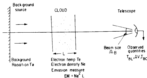
Figure 3. Schematic model used for interpretation of recombination lines in the direction of blank regions and SNRs.
