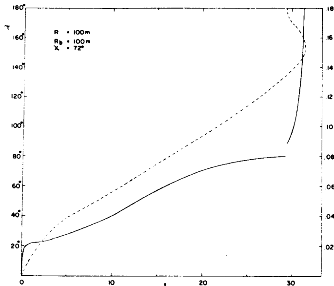
Figure 2 b. The figure shows that the dashed curve t(\psi) develops a maximum but remains finite. The undashed curve I(t) implies that the flux profile has a discontinuity and terminates in a burst.
