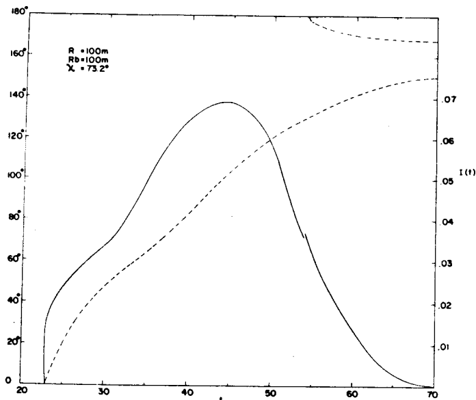
Figure 2 c. The dashed curve t(\psi) tends to infinity as \psi approaches the critical values \psi_1 and \psi_2 . The undashed curve I(t) possesses a maximum and a discontinuity, which is smaller in height in comparison to case (b). The flux strength finally decays as t tends to infinity.
