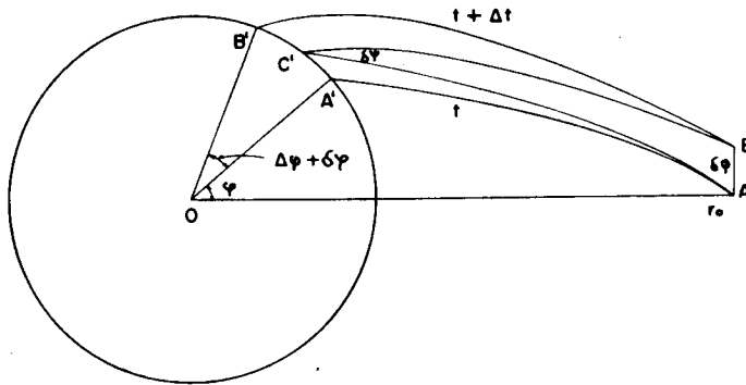
Figure 1. The figure shows the null geodesics emanating from A' and B' which reach A and B at times t and t + \Delta t respectively. The points A' and B' lie on the shell R = R_b , which has neutrino sources distributed uniformly over it. AB is the elemental area at r = r_0 at the point of observation. C' is a typical point lying between A' and B' which emits neutrinos that pass through AB in a very small time interval lying between t and t + \Delta t . The angles \Delta\varphi + \delta\varphi subtended by the arc A'B' at O and \delta\psi between C'B and C'A have been exaggerated for the sake of clarity in the diagram.
