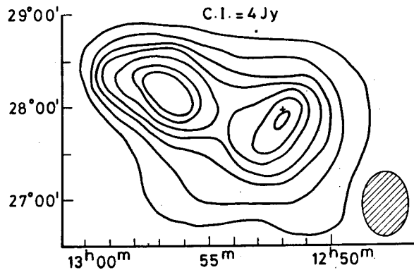
Figure 2. Map of the Coma cluster region after subtraction of the point sources 5C 4.81 and 5C 4.85. The position of the radio galaxy Coma A is shown by a cross.
