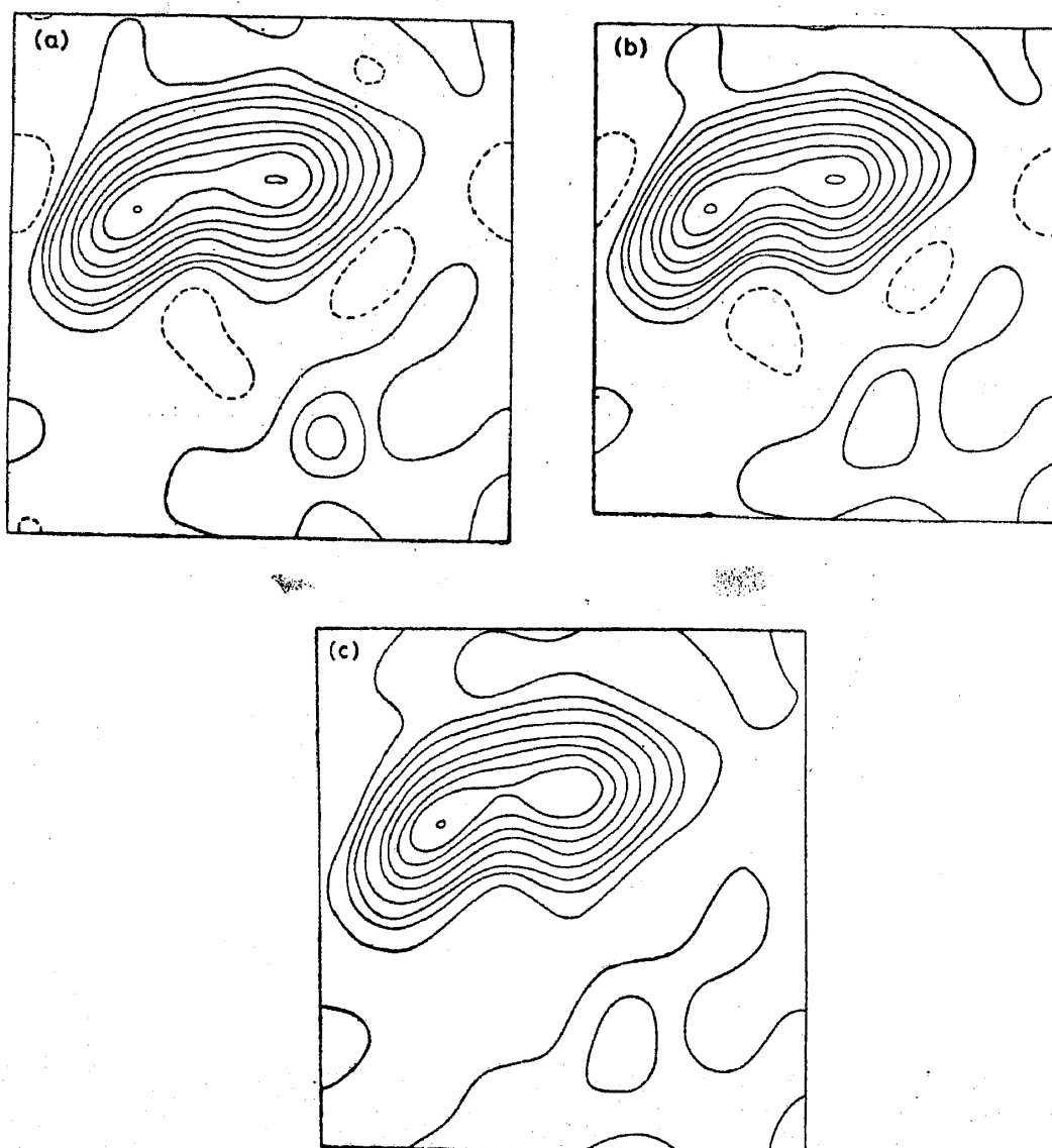
Figure 14. Illustration of the different ways of treating noisy data with the MEM. (a) R = 100 , -B \ln B MEM map of Fig. 9b with gaussian noise of rms = 1 added to the Fourier coefficients \rho_{mn} , |m|, |n| \leq 3 ; (b) -B \ln B MEM restoration from the noisy data in (a) with R = 100 , fitting the data exactly; (c) -B \ln B MEM restoration fitting the data in (a) by the least-squares method with \sigma = 1 . Note that the result is not less noisy than (b) but has rounded off the peaks and distorted the ripple so that it no longer goes negative.
