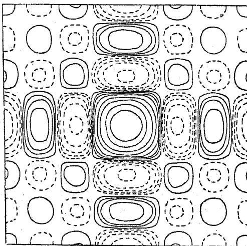
Figure 5. The reconstruction of a point source using only Fourier coefficients \rho_{mn} with |m|, |n| \leq 3 . This is the so-called dirty beam. Negative contours are shown by broken lines.
