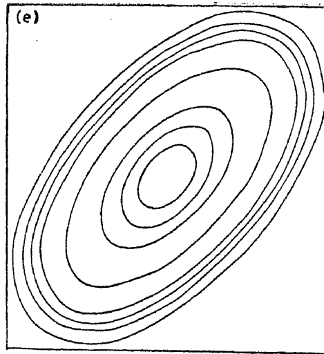
Figure 12. (e) Restoration with a modified entropy \ln(B + C_1) + \ln(C_2 - B) with C_1 and C_2 FLOATING constants determined by (B_{\max} + C_1)^2 / (B_{\min} + C_1)^2 = 100 , B_{\min} + C_1 = C_2 - B_{\max} . With this entropy the ripple has disappeared both from the low-lying region and the plateau.
