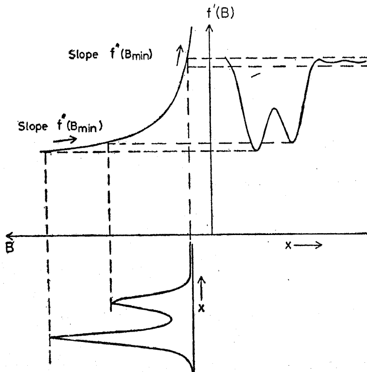
Figure 1. Illustration of the peak-sharpening and baseline-flattening properties of the MEM. The case shown is f(B) = \ln B . According to Equation (7), f'(B) = 1/B is a band-limited function, shown to the right of the vertical axis. The function shown below is B . It is clear that the large slope [ f''(B) ] of the curve of f'(B) vs. B at small B ensures a flat baseline, and the small slope at large B ensures sharp peaks.
