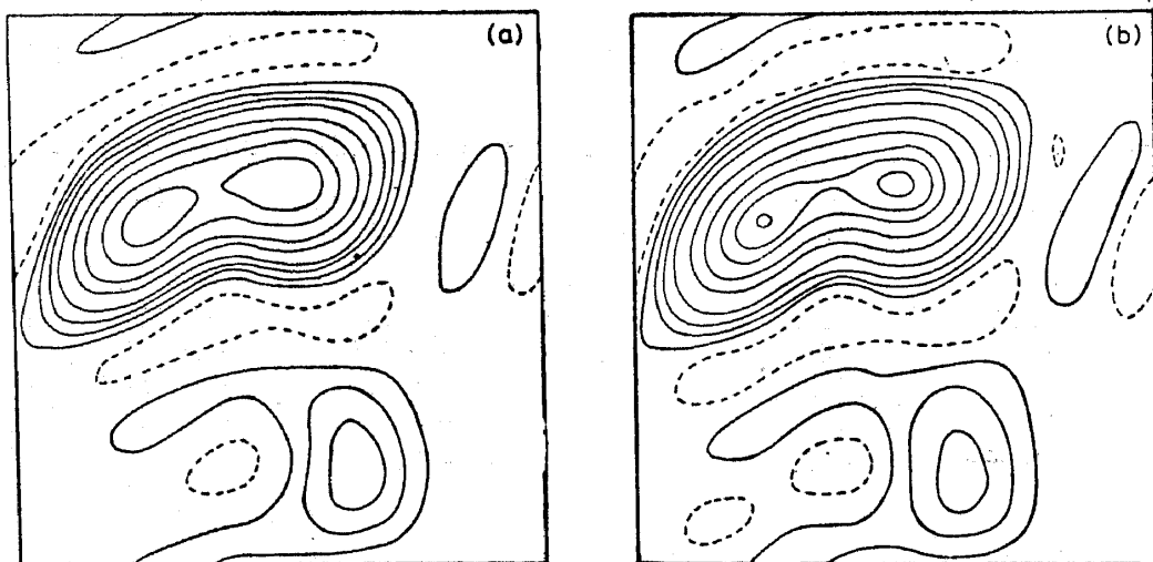
Figure 11. Reconstruction from the data of Fig. 6 using (a) a very 'soft' entropy -B^{3/2} with R = 100 (note the ripple in the baseline and rounded peak), (b) a very hard entropy -\exp(-aB) with R = 25 ; note the very sharp peaks and rippled baseline.
