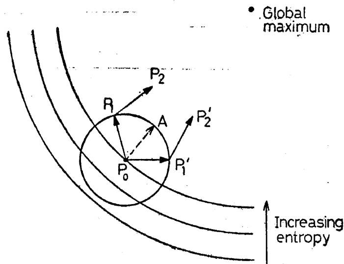
Figure 13. The space of measured Fourier coefficients. P_0 represents the true values, while P_1, P_1' etc. represent the values that would be obtained in measurements with different realisations of the noise. P_1, P_1' etc. lie on a sphere of radius \sigma\sqrt{2N} where 2N is the number of (real) measurements and \sigma the rms of each. Starting from the noisy data, P_1, P_1' etc. the least-squares approach moves a distance \sigma\sqrt{2N} to P_2, P_2' etc. The average over all realisations of the MEM solutions P_2, P_2' etc. is the point A which has a systematic and predictable bias P_0A from the true data. The vectors P_1P_2, P_1'P_2' represent the residuals and, for small \sigma , are independent of position on the sphere, pointing in the direction of increasing entropy, perpendicular to the constant entropy contours. At the centre of these contours is the unconstrained maximum entropy solution viz. a flat map ( \rho_{00} is assumed fixed).
