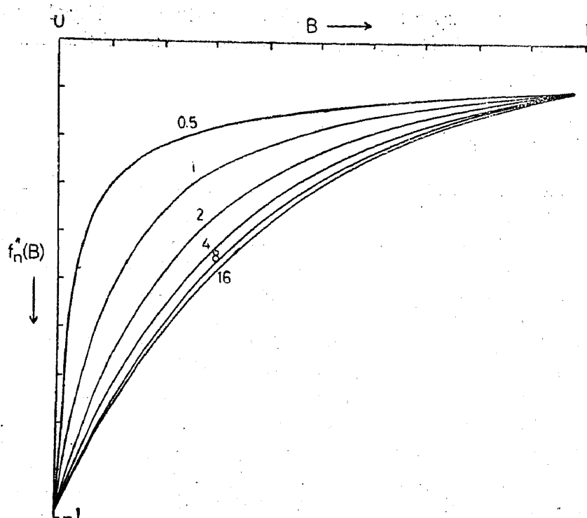
Figure 2. Variation of f''(B) vs. B for various entropies characterised by f'' = 1/(B + C)^n . f'' varies from -10 to -1 as B varies from 0 to 1 . The values of n go from 0.5 to 16 and are indicated against the corresponding curves. Note that all the entropies with large n tend to a single curve (corresponding to the exponential entropy f = -e^{-\alpha\beta} ). The 'softer' entropies with smaller values of n produce a flatter baseline and blunter peaks than the 'hard' entropies with large n .
