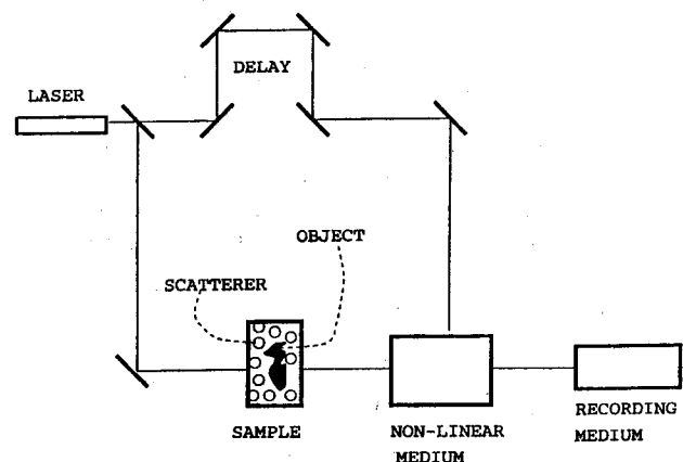
Figure 3. Schematic diagram of an experiment to image through turbid media using a nonlinear process for discrimination.
