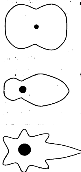
Figure 1. Intensity distribution of scattered light of wavelength \lambda from a spherical particle of radius a . a < \lambda ; b , a = \lambda/4 ; and c , a > \lambda .
