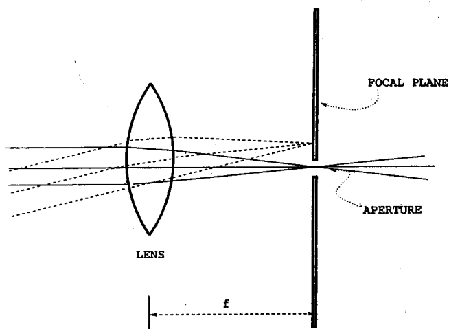
Figure 7. A spatial filter formed by a lens and an aperture at its focal point.
