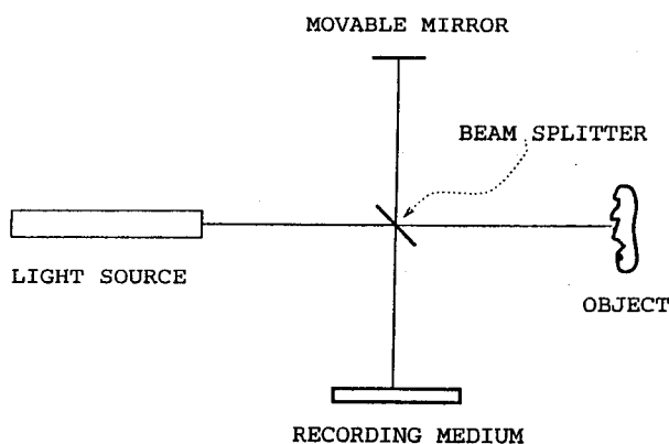
Figure 6. Schematic diagram for optical coherence tomography.
