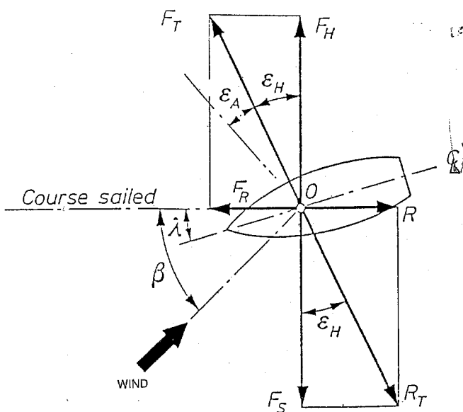
Figure 10. Lanchester's Course Theorem. The closest angle \beta to the wind that a craft can sail is the sum of the under and above water gliding angles.
