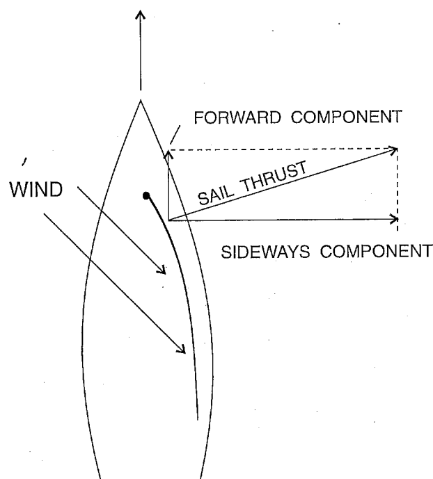
Figure 8. Force components of the sail thrust when going into the wind. The large sideways component must be countered by an underwater arrangement.
