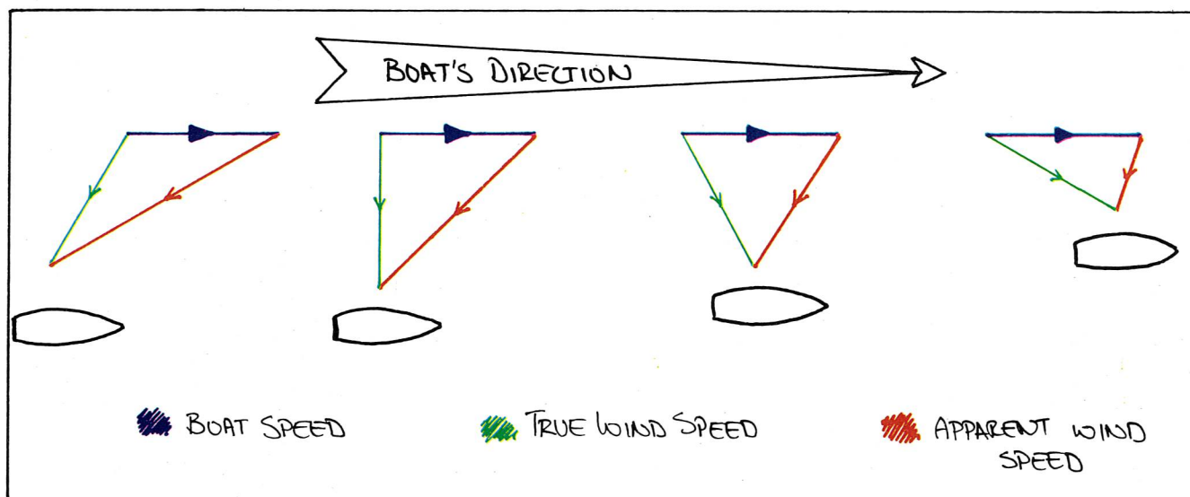
Figure 13. True and apparent winds. The apparent wind can be less than, equal to, or greater than the true wind depending on the point of sailing. The boat speed has been kept constant in all cases in this illustration.
