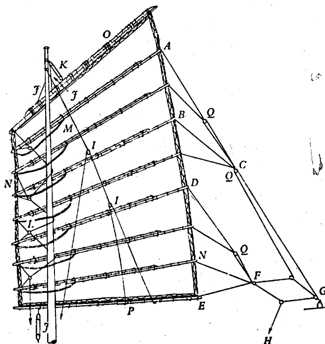
Figure 7. A Chinese mainsail, which could be hoisted or lowered from on deck by one person.
