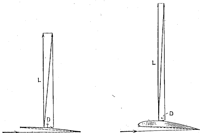
Figure 9. Lift and drag on curved plate (left) and airfoil (right) at an angle to the wind of under 4 degrees. Both have the same aspect ratio of 6.
