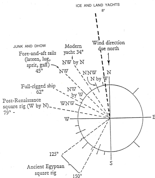
Figure 11. The closest angle to the wind, \beta , for sailing vessels through the ages. Ice and land yachts can sail very close to the apparent wind because they have a very high ratio of lateral to forward resistance.
