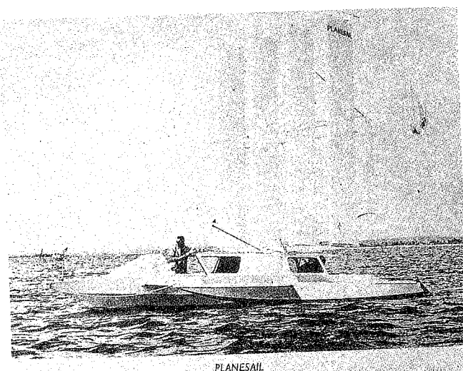
Figure 23. John Walker's first wingsail trimaran built over a quarter century ago had four main wings. The tail controlling their angle to the wind can be seen behind them.
