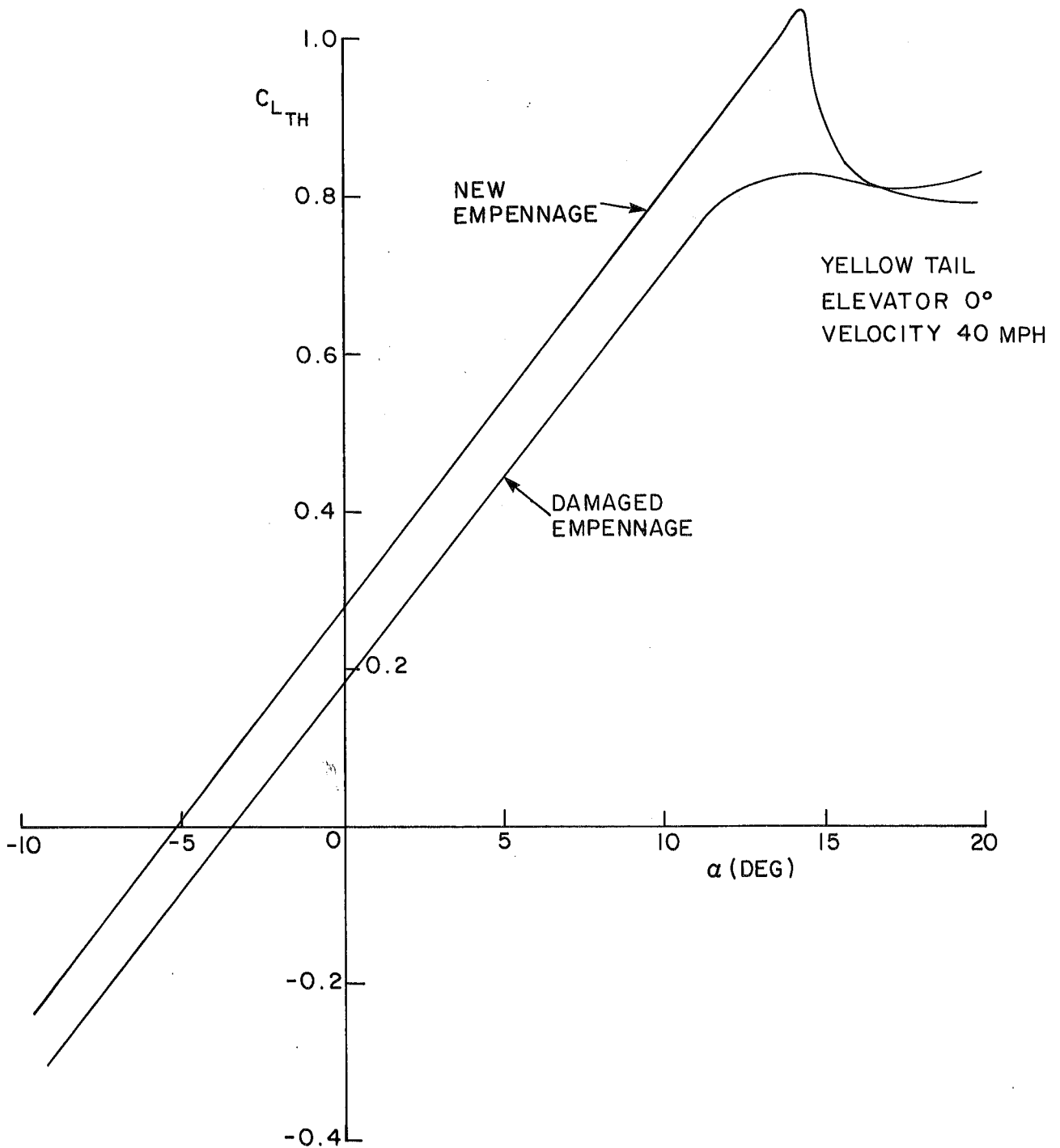
FIG. 14: DAMAGED TAIL ASSEMBLY
