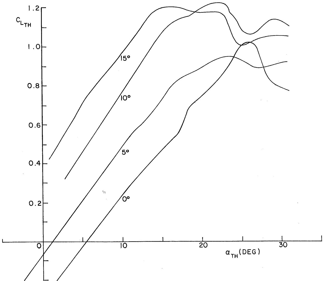
FIG. 12: C_{LTH} VERSUS \alpha_{TH} FOR \delta_e VARIED
