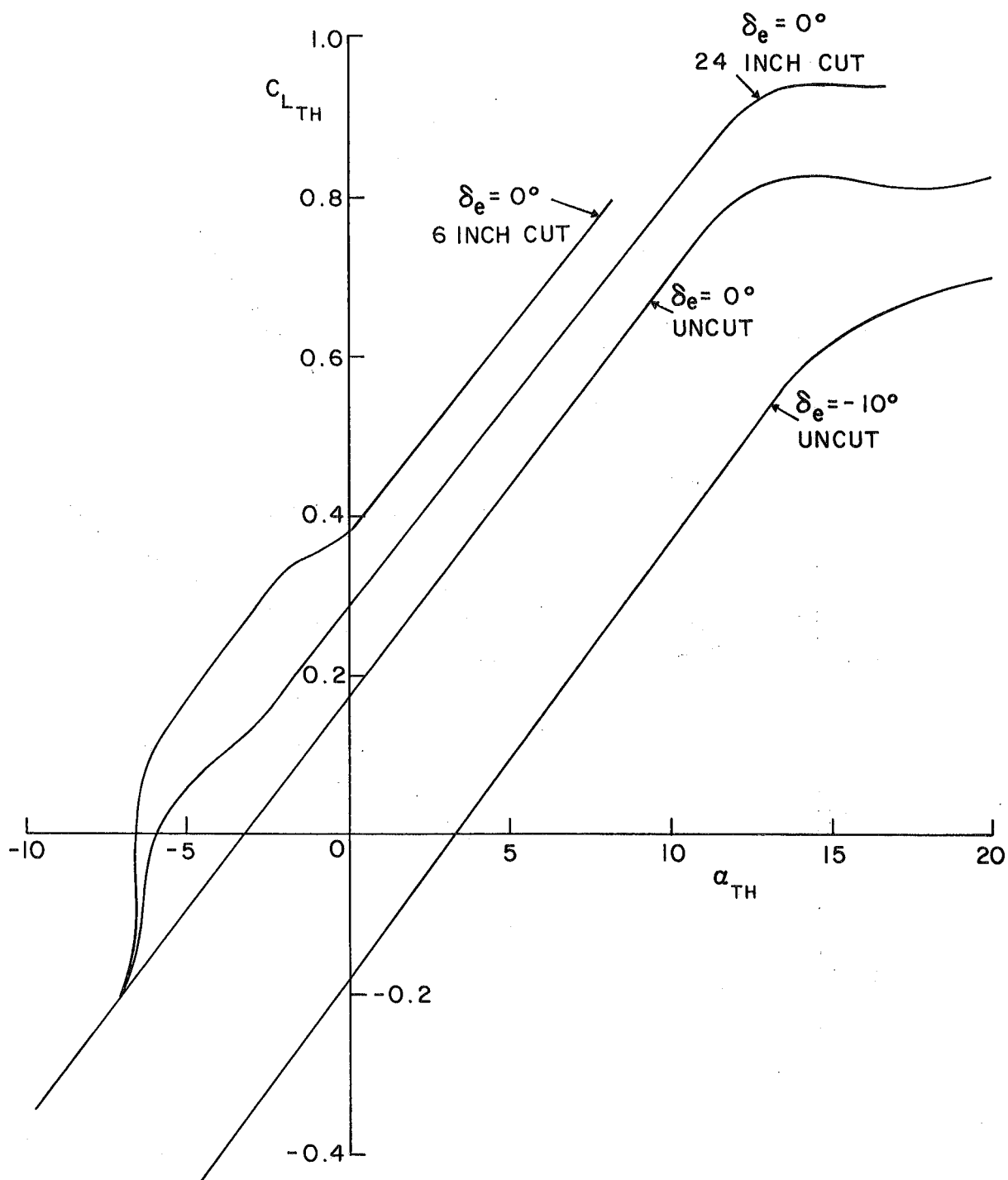
FIG. 15: CUT FABRIC C_{LTH} VERSUS \alpha_{TH}
