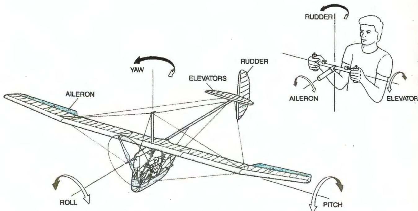
THREE-AXIS CONTROL of a typical third-generation craft is achieved solely with the pilot's hands. (His legs are pedaling to pro-
