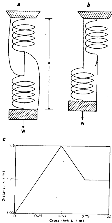
Figure 2. A spring-string system. a , With the central link string intact, the support strings are limp. b , Without the central link string, the weight gets lifted up for a certain range of lengths of the central string. c , Variation of distance X from the support to the weight for different lengths L of the central link string.
