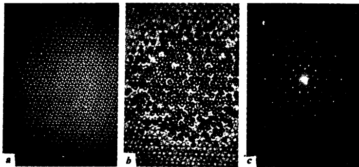
Figure 2. Optical quasicrystal. a. A 2D quasicrystal lattice due to five equally inclined laser beams; b. condensation of spheres; c. the associated diffraction pattern. [From Burns, M. M., Fournier, J.-M. and Golovchenko, J. A., Science , 1990, 249, 749]
