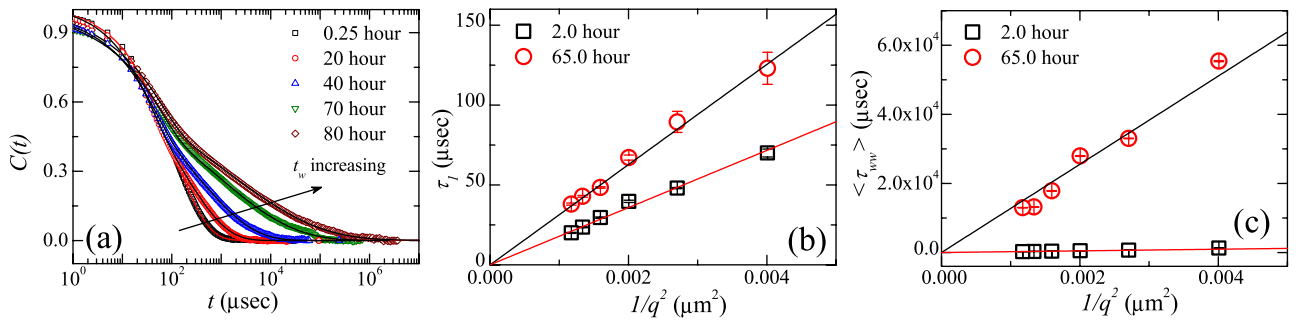
FIG. 1. (a) The normalized intensity autocorrelation functions C(t) , vs. the delay time t , at 25 °C and scattering angle \theta = 90^\circ , for 2.5% w/v Laponite suspension with 0.05 mM salt at several t_w . The solid lines are fits to Equation (1). The diffusive behavior of the fast relaxation time ( \tau_1 ) and the mean slow relaxation time ( \langle\tau_{ww}\rangle ) are shown in (b) and (c), respectively, for a 2.5% w/v Laponite suspension. The solid lines are linear fits passing through the origin.
