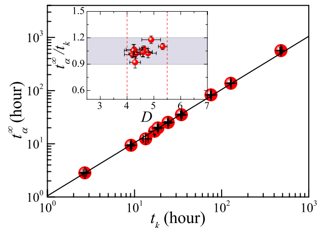
FIG. 4. Analogous Vogel time t_\alpha^\infty is plotted vs. t_k , the waiting time at which \beta \rightarrow 0 . Solid line is the linear fit with a slope 1.02 \pm 0.025 . In the inset, the ratio t_\alpha^\infty/t_k is plotted vs. D .
