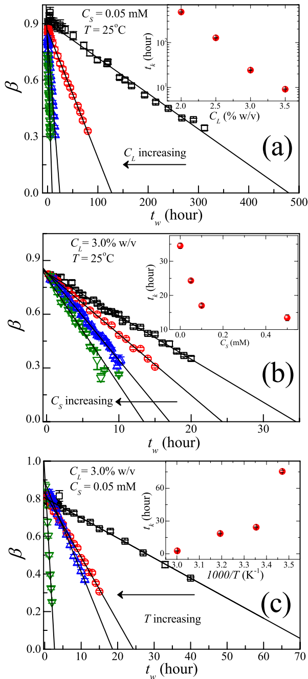
FIG. 3. (a) Stretching exponents \beta are plotted vs. t_w for C_S = 0.05 mM and T = 25^\circ\text{C} at different C_L (from right to left, 2.0% w/v ( \square ), 2.5% w/v ( \circ ), 3.0% w/v ( \triangle ), 3.5% w/v ( \nabla )). (b) \beta vs. t_w for C_L = 3.0\% w/v and T = 25^\circ\text{C} at different C_S (from right to left, 0 mM ( \square ), 0.05 mM ( \circ ), 0.1 mM ( \triangle ), 0.5 mM ( \nabla )). (c) \beta vs. t_w for C_L = 3.0\% w/v and C_S = 0.05 mM at different T (from right to left, 15^\circ\text{C} ( \square ), 25^\circ\text{C} ( \circ ), 40^\circ\text{C} ( \triangle ), 60^\circ\text{C} ( \nabla )). t_k ( \bullet ), the waiting times at which \beta \rightarrow 0 , measured by extrapolating of \beta to 0, are plotted for different C_L , C_S , and T in the insets of (a), (b), and (c), respectively.
