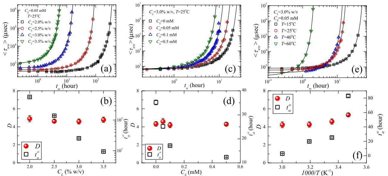
FIG. 2. Mean slow relaxation times \langle\tau_{ww}\rangle , obtained by fitting C(t) data to Equation (1), are plotted vs. t_w for different C_L , C_S , and T in (a), (c), and (e), respectively. Fragility D ( \bullet ) and Vogel time t_\alpha^\infty ( \square ), measured by fitting \langle\tau_{ww}\rangle data to the Equation (2), are plotted for different C_L , C_S and T in (b), (d), and (f), respectively.
