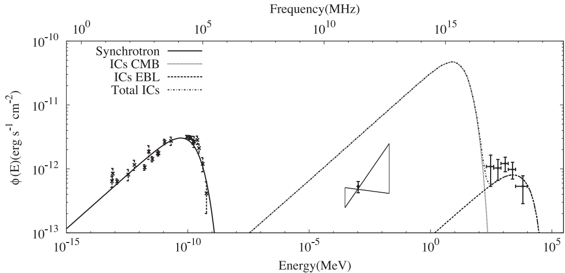
Figure 9. The broad-band SED of Fornax A for Model I, where both the X-rays and \gamma -rays are produced by IC scattering by the synchrotron-emitting electrons. The IC scattering contribution from the EBL and the CMB photon fields are both shown in the figure. The model parameters are described in Table 2.
