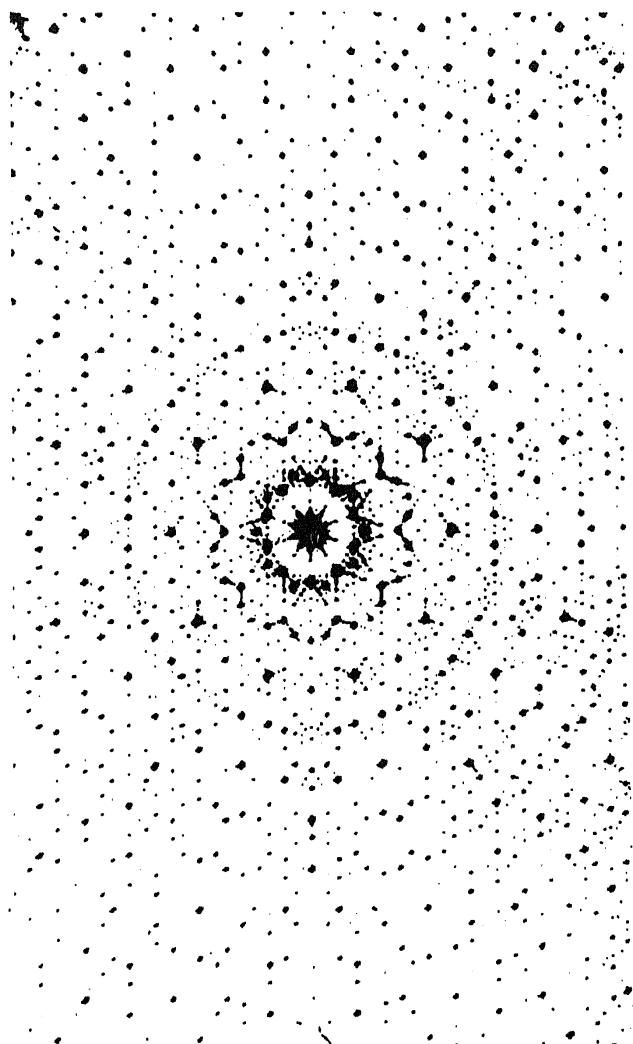
Figure 6. Optical transform of a two-dimensional Penrose tiling pattern (after Mackay 4 ).
