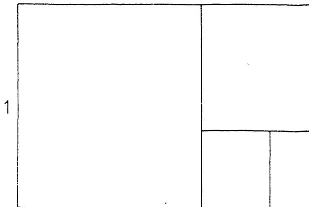
Figure 3. The golden mean of the Greeks.
