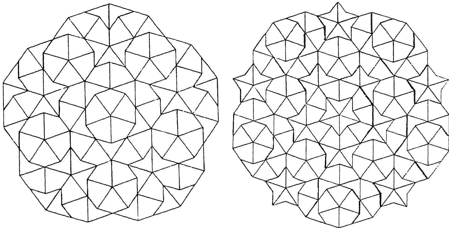
Figure 5. Two non-periodic Penrose patterns.
