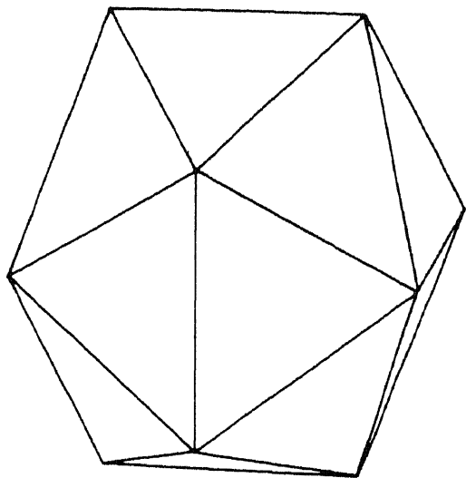
Figure 2. The icosahedron—one of the Platonic solids.
