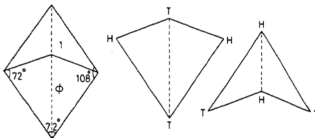
Figure 4. Two basic tiles of Penrose.
