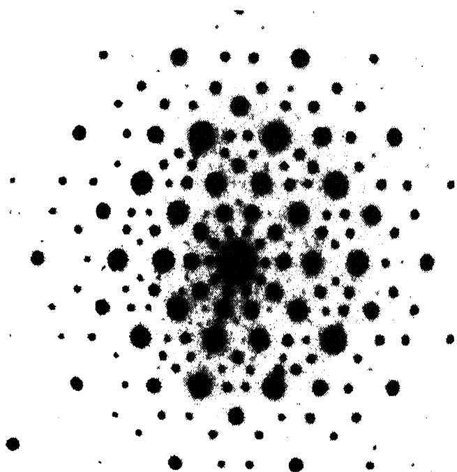
Figure 8. Electron diffraction pattern of supercooled Al-Mn alloy showing icosahedral symmetry.
