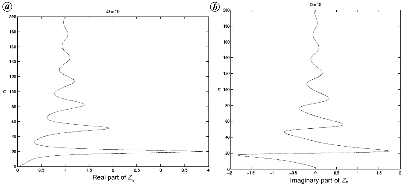
Figure 3. a , Iteration of the two-terminal network impedance ( \text{Re } Z_n(\omega) ) initialized at Z_0 = 0.05 + i0 . Note the fast convergence to the stable fixed point Z_n^* = 1 . Here R = L = C = 1 , and \omega = 10 . b , Iteration of the two-terminal network impedance ( \text{Im } Z_n(\omega) ) initialized at Z_0 = 0.05 + i0 . Note the fast convergence to the stable fixed point Z_n^* = 1 . Here R = L = C = 1 and \omega = 10 .
