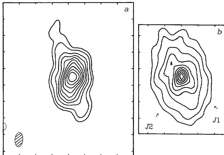
FIG. 2.—A CLEAN image ( a ), and an equivalent image produced with a maximum-entropy convolution algorithm ( b ), of 0316+413 at 7 mm wavelength at epoch 1987 June 10–11. The contours are at -3, 5, 10, 20, \dots, 80 , and 90% of the peak brightness, 3 Jy per beam area for image ( a ). The 50% contour of the restoring beam for the CLEAN image with a FWHM size of 100 \times 170 \mu\text{as} and a position angle of -7^\circ is shown as a striped ellipse in the lower left corner of ( a ). Tick marks in both images are separated by 200 \mu\text{as} . North is up, and east to the left.
