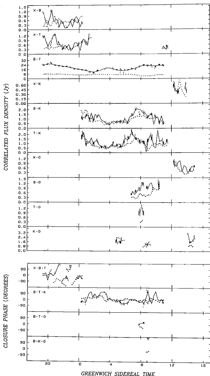
FIG. 1.—Correlated flux densities and closure phases for 0316+413 shown with \pm 1\sigma statistical standard errors. Nondetections, caused by sensitivity limitations, are not plotted. The solid lines represent the predictions from the CLEAN components used to produce the image shown in Fig. 2a. The dotted lines show the predictions from the equivalent components from the image at epoch 1986 May 9–10.
